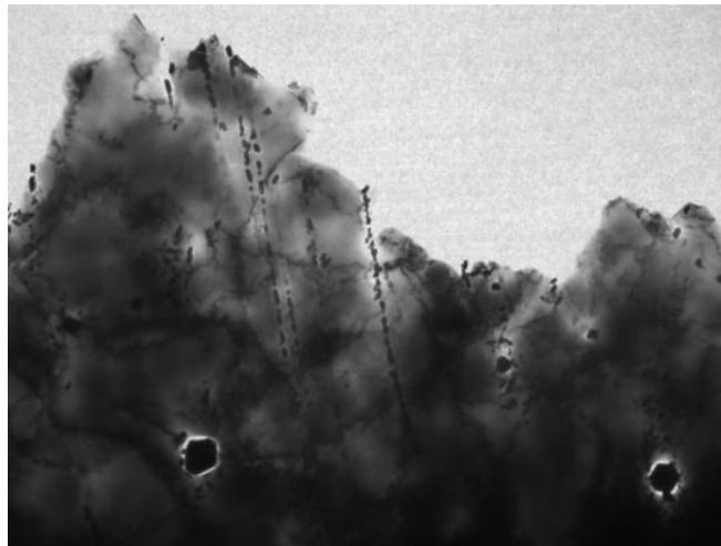
Figure 3.30 Rows of smaller carbides aligning into grain boundaries in Haynes 230 deformed at 600 °C and 10^{-3} \text{ s}^{-1}
